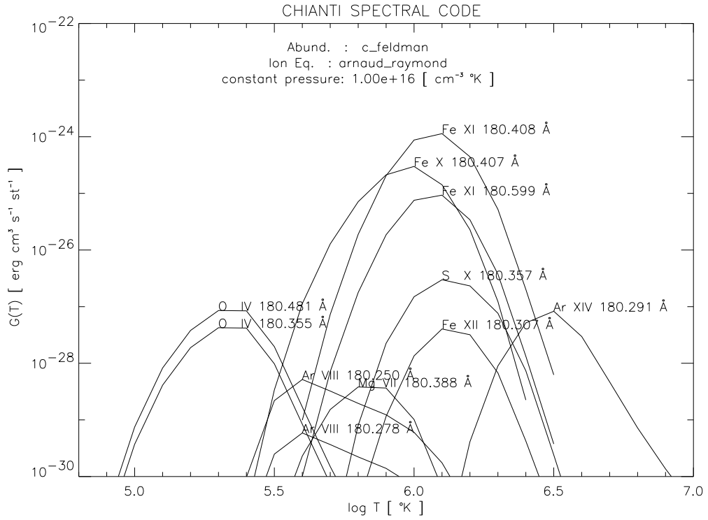
Figure 9: One of the G(T) plot of the test case
