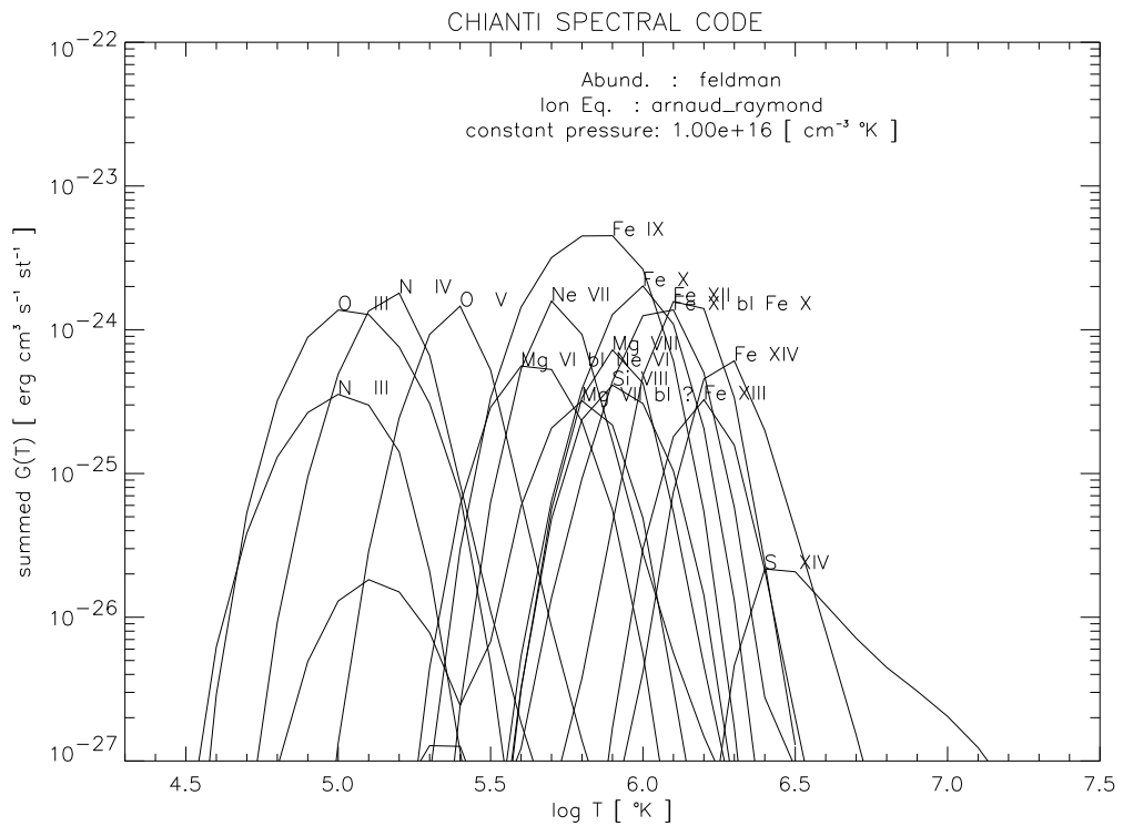
Figure 10: The summed- G(T) plot of the test case: test_gt.ps
